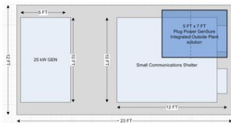
58% FOOTPRINT SAVINGS USING PLUG POWER'S GENSURE INTEGRATED OSP SOLUTION COMPARED TO A SMALL COMMUNICATIONS CABINET AND COMBUSTION GENERATOR
